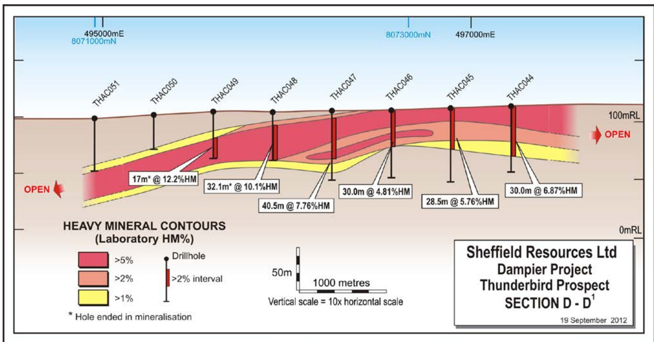
Figure 4: Cross-section D-D' through the Thunderbird HMS deposit
